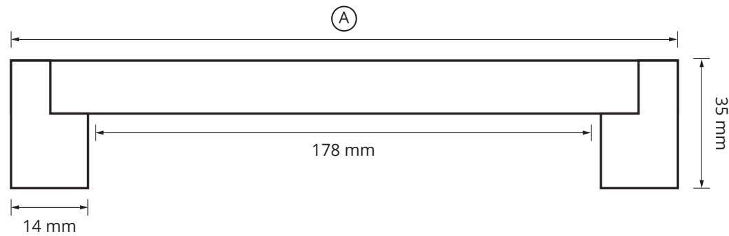
VISTA FRONTAL
